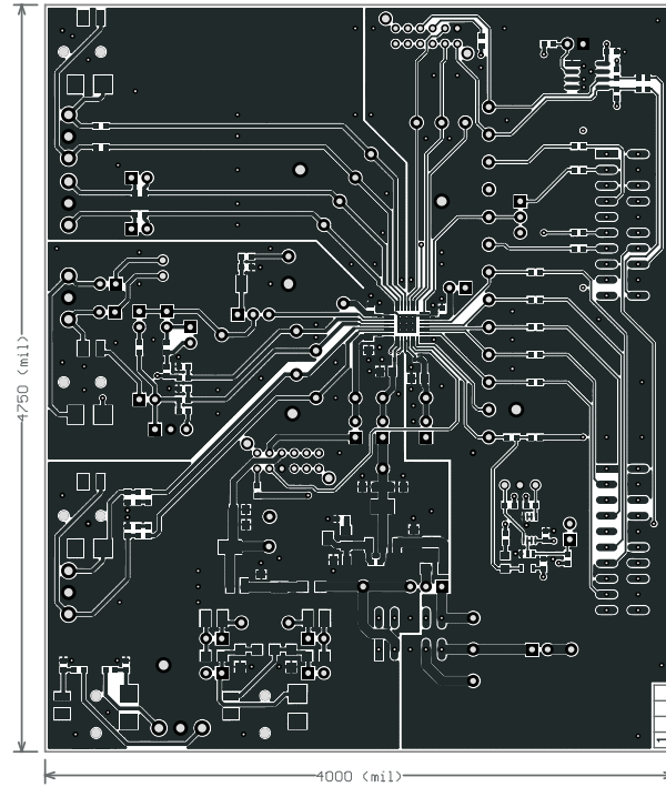
Figure C-1. Top Layer
