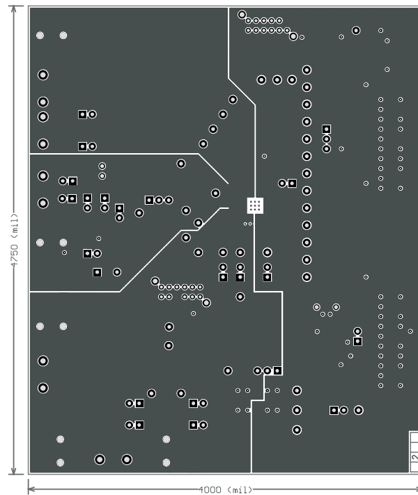
Figure C-2. Mid-Layer 1
