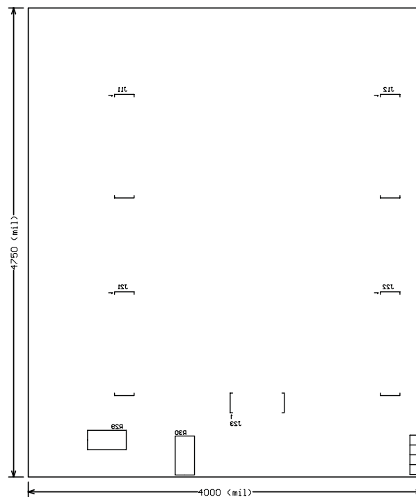
Figure C-6. Bottom Overlay
