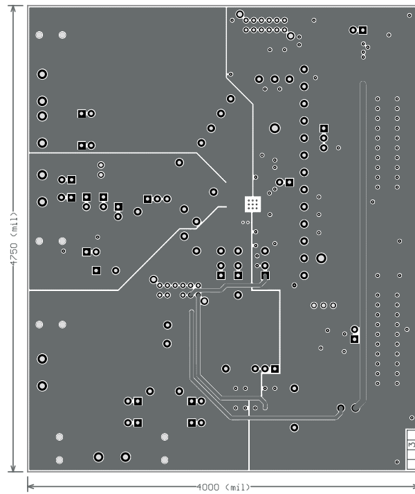
Figure C-3. Mid-Layer 2
