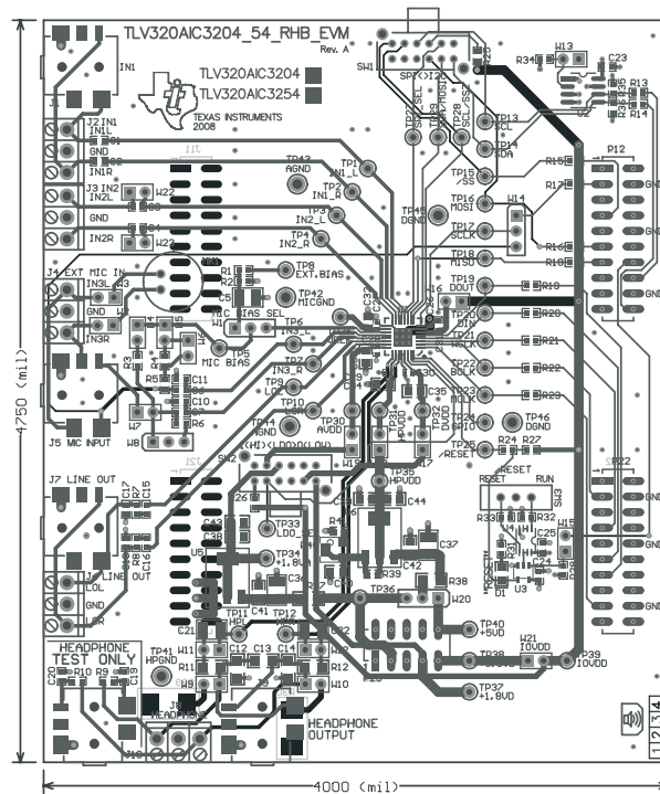
Figure C-8. Composite
