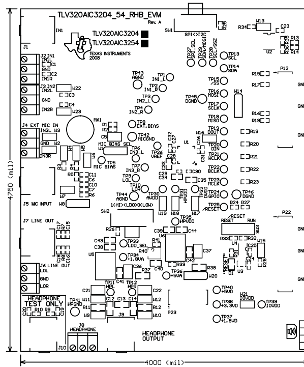
Figure C-5. Top Overlay
