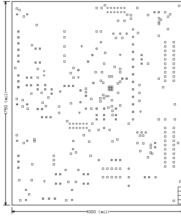
Figure C-7. Drill Drawing
